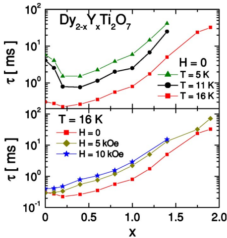
FIG. 9. The characteristic spin relaxation time as a function of dilution for \text{Dy}_{2-x}\text{Y}_x\text{Ti}_2\text{O}_7 at T = 5, 11, and 16 K in zero field, and at H = 0, 5, and 10 kOe at T = 16 K. A minimum is evident near x \sim 0.4 for low temperatures and small fields.
